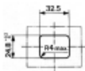
Snap-in Mount
