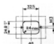
Screw Mount
