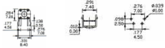
Drilling Pattern
