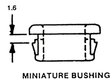
MINIATURE BUSHING
