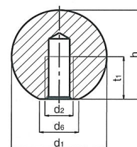
Moulded thread – M i.e. 11-KPBG20M5
