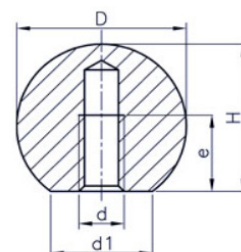
Moulded thread – M i.e. 11-KPBB16M4
