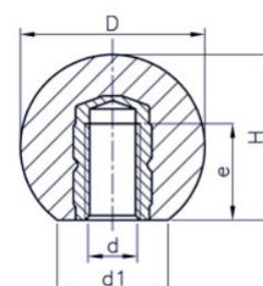
Brass Insert – B i.e. 11-KPBB16B4
